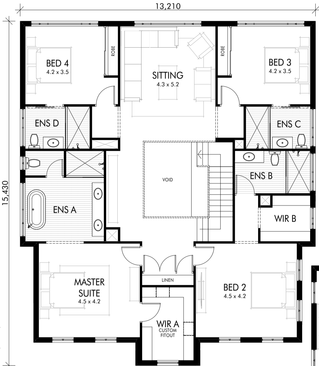
UPPER FLOOR PLAN
